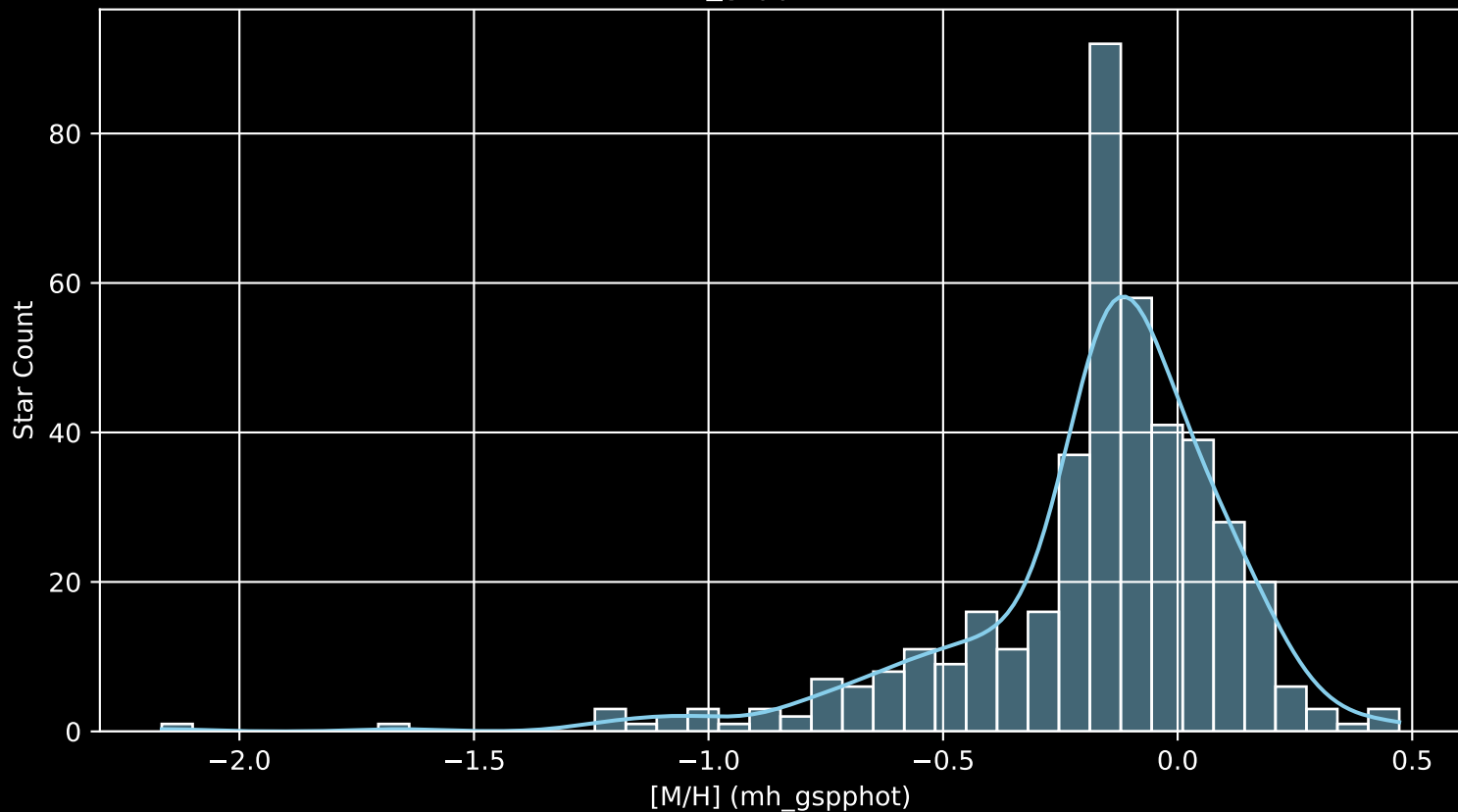
APOGEE DR17 Field: [120-08 [M/H] (mh_gspphot) (n= 429)
