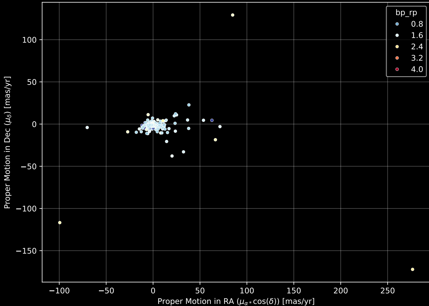
APOGEE DR17 Field: [120-08] Proper Motion Diagram (n= 433)
