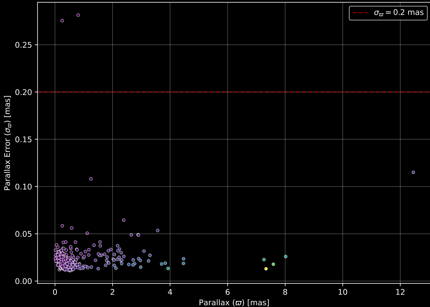
APOGEE DR17 Field: [120-08] Parallax Quality (n= 433)
