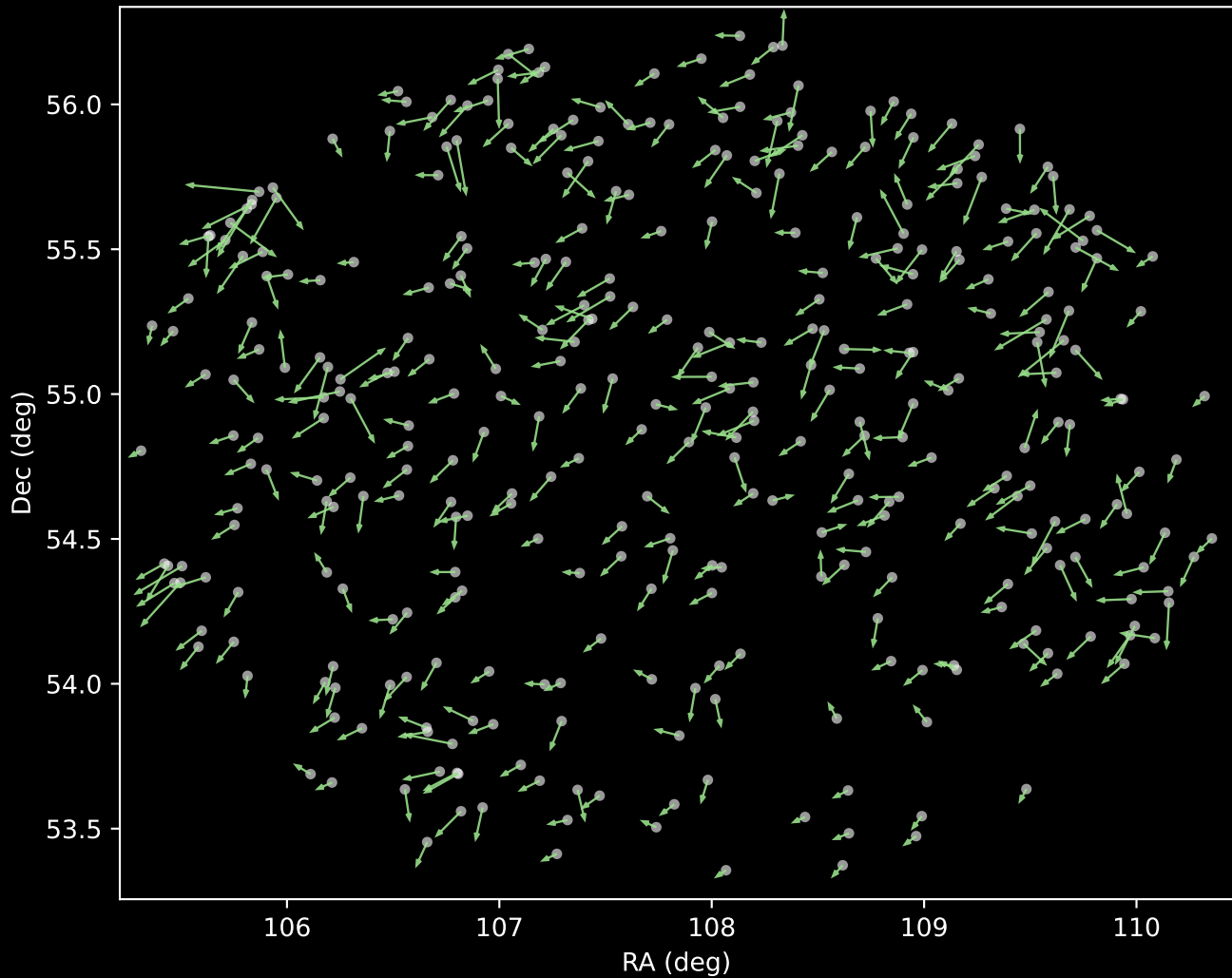
APOGEE DR17 Cluster 5 Proper Motion Vectors (n=354)
