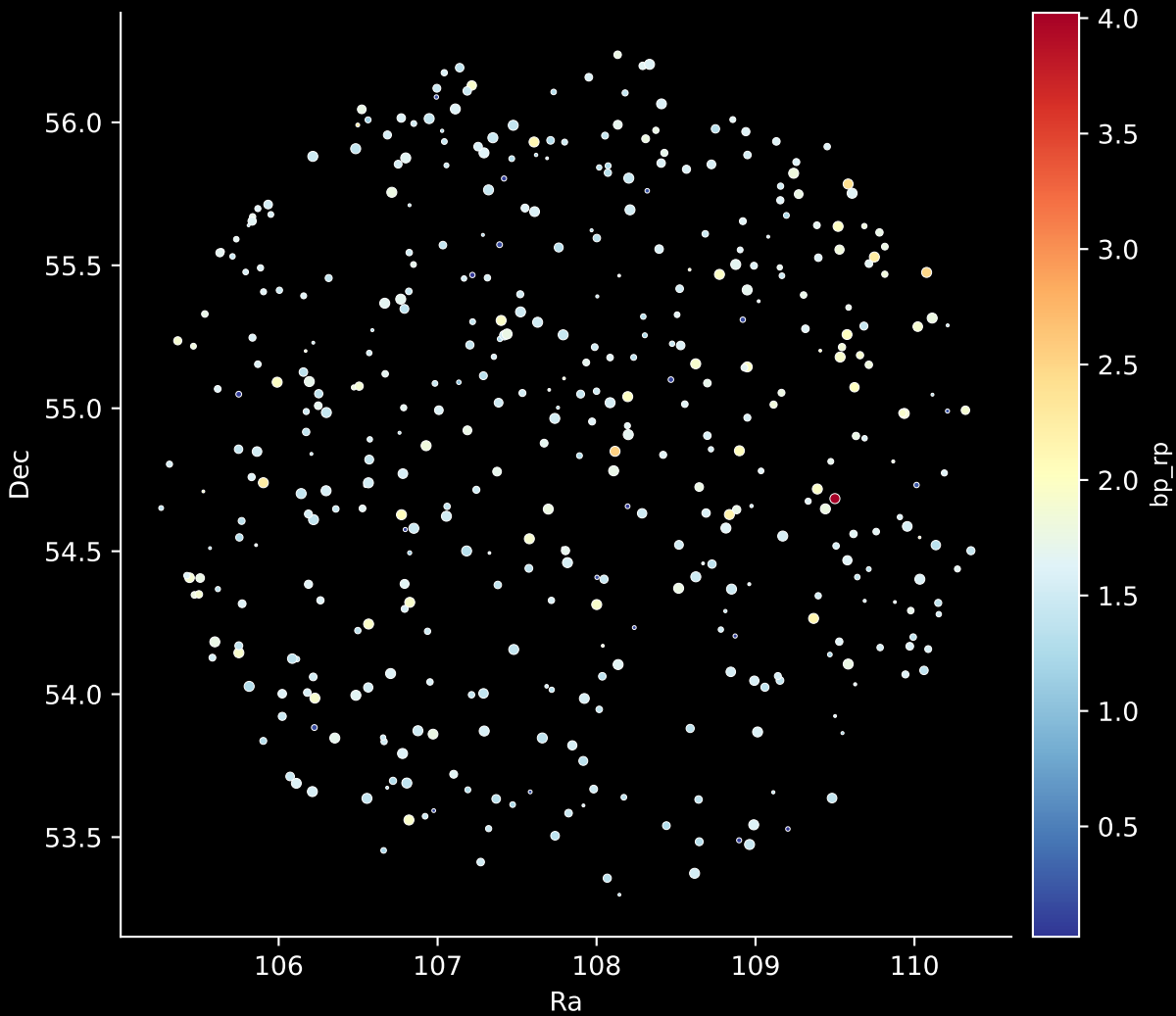
APOGEE DR17 Field: [120-08] Stars: 433
