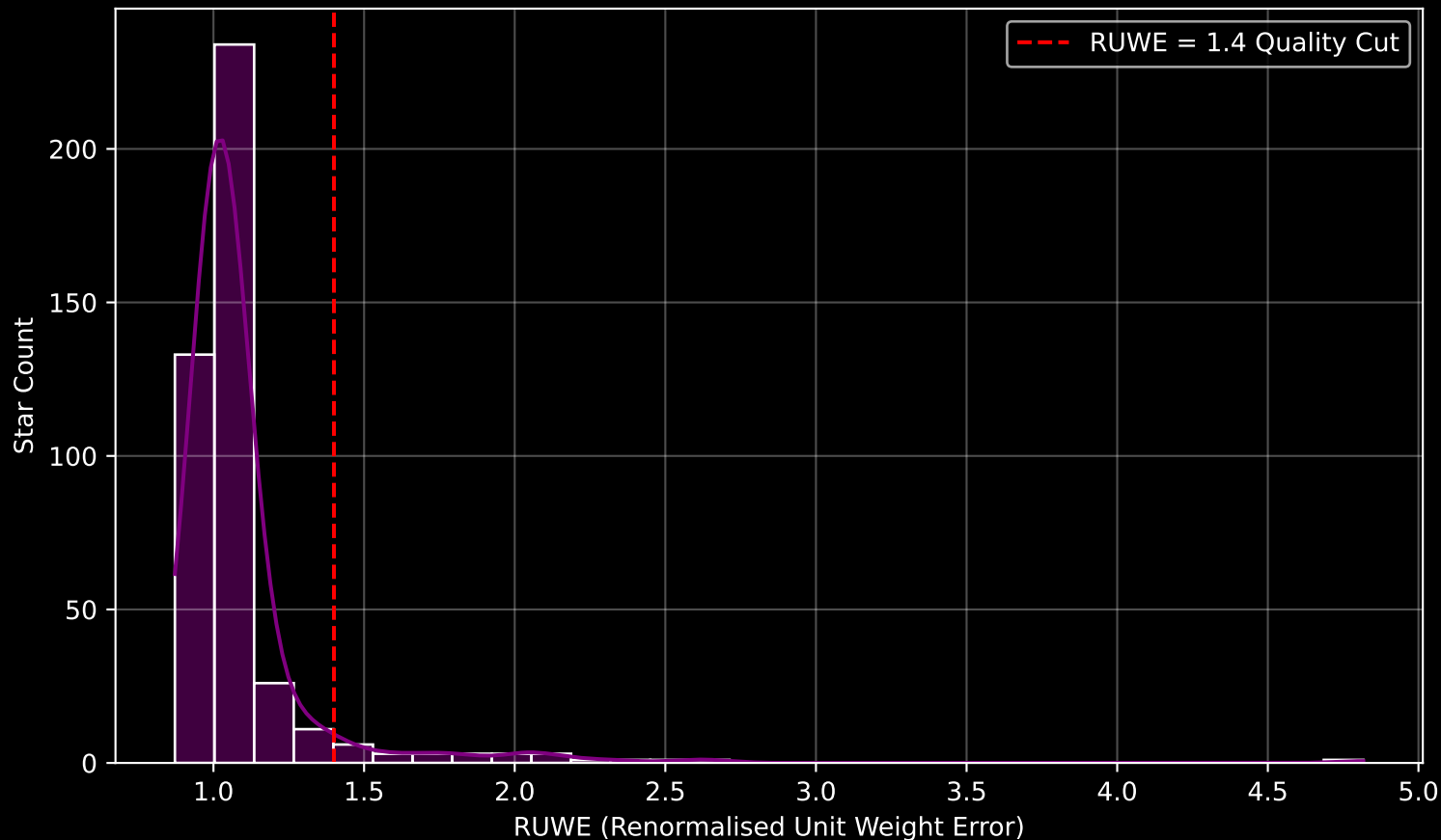
GAPOGEE DR17 Field [120-08] RUWE Distribution (n= 430)
